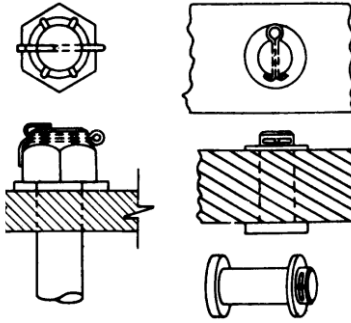
FIGURE 7-6. Securing with cotter pins.
