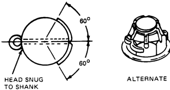
FIGURE 7-7. Alternate method for securing with cotter pins.
