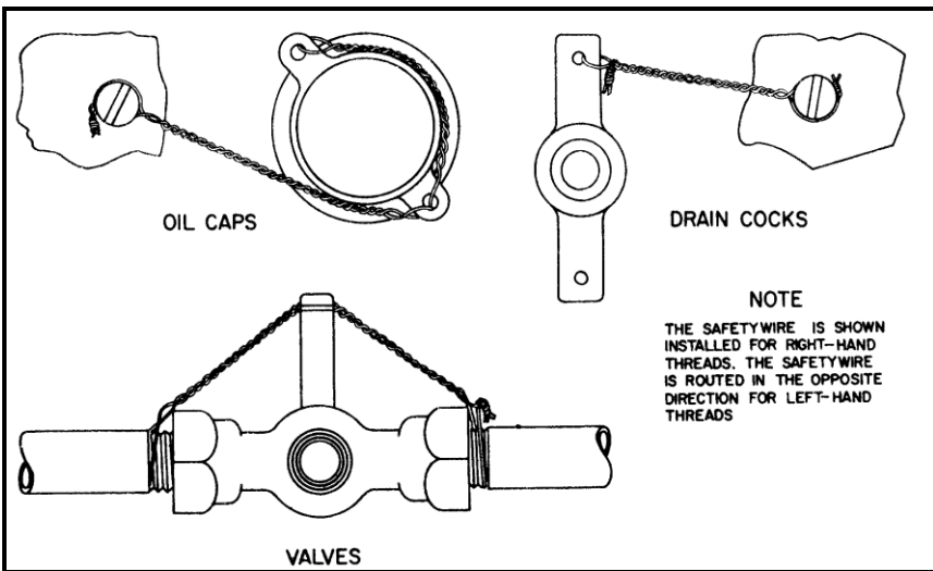
FIGURE 7-4a. Securing oil caps, drain cocks, and valves.
