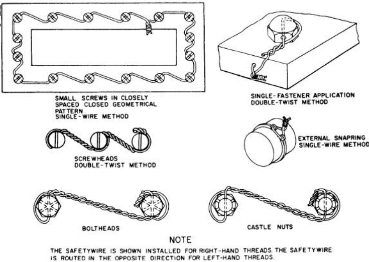
FIGURE 7-3. Securing screws, nuts, bolts, and snaprings.
